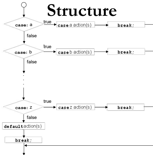
Fig. 5.11 Flowcharting the switch multiple-selection structure.
