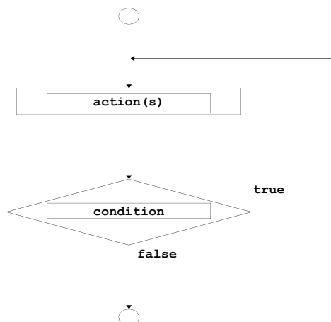
Fig. 5.13 Flowcharting the do/while repetition structure.
