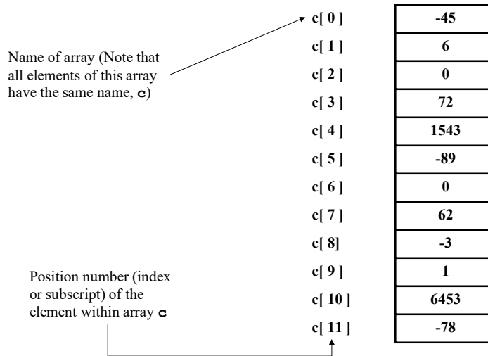
Fig. 7.1 A 12-element array.
