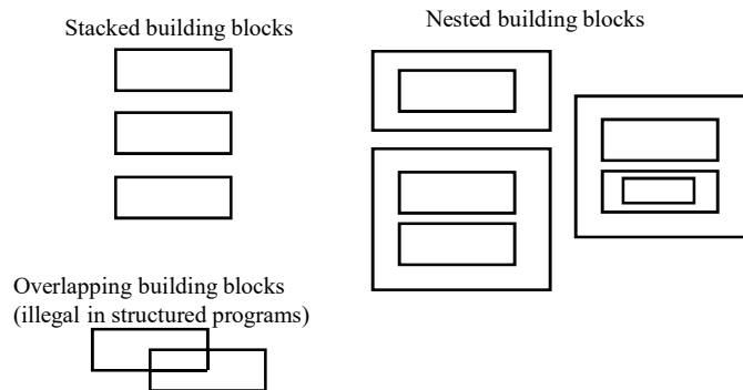
Fig. 5.27 Stacked, nested and overlapped building blocks.
